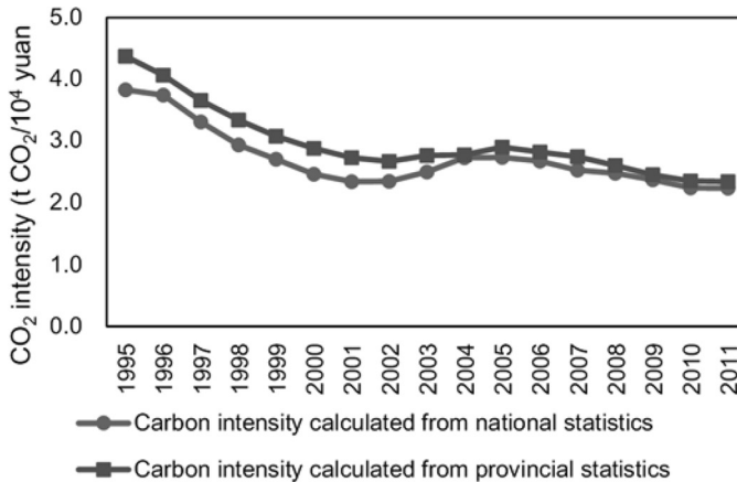
Figure 5: CO 2 intensity calculated from provincial and national statistics
